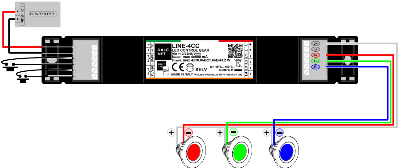
Figure 4: Wiring diagram for RGB load
