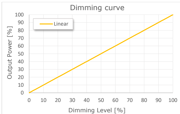
Figure 11: Dimming Curves
