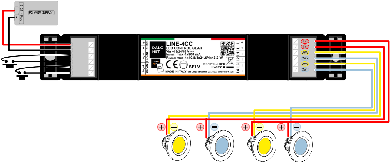
Figure 3: Wiring Diagram for Tunable-White LED Loads
