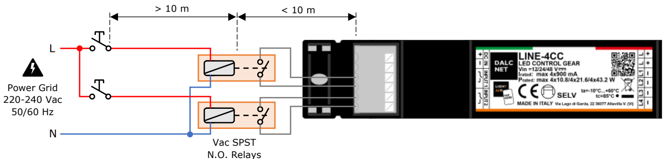
Figure 7: Connecting the Local Command for Long Distances
